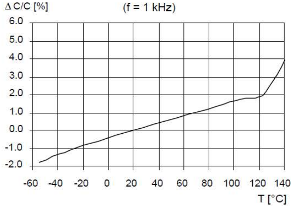
Capacitance vs. temperature
