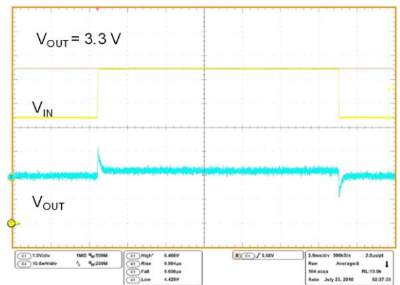
Figure 18: Line transient
