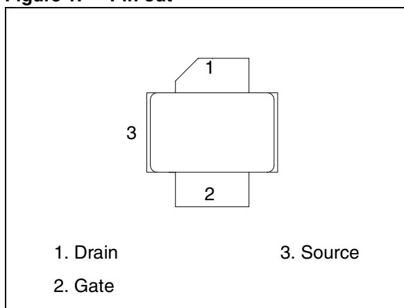
Figure 1. Pin out
