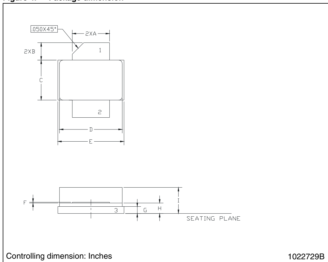
Figure 4. Package dimension
