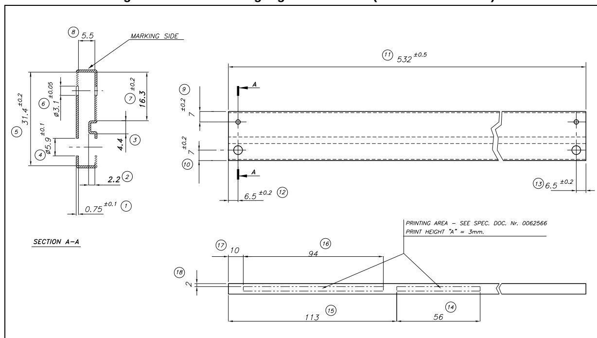
Figure 20. TO-220 single gauge tube outline(dimensions in mm)
