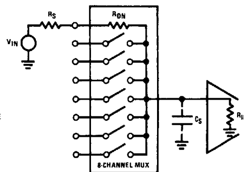
FIGURE 6. 8-Channel MUX
