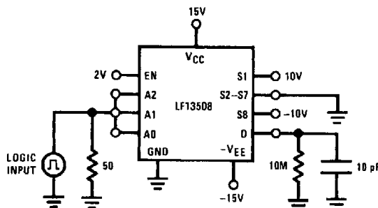
FIGURE 1. Transition Time
