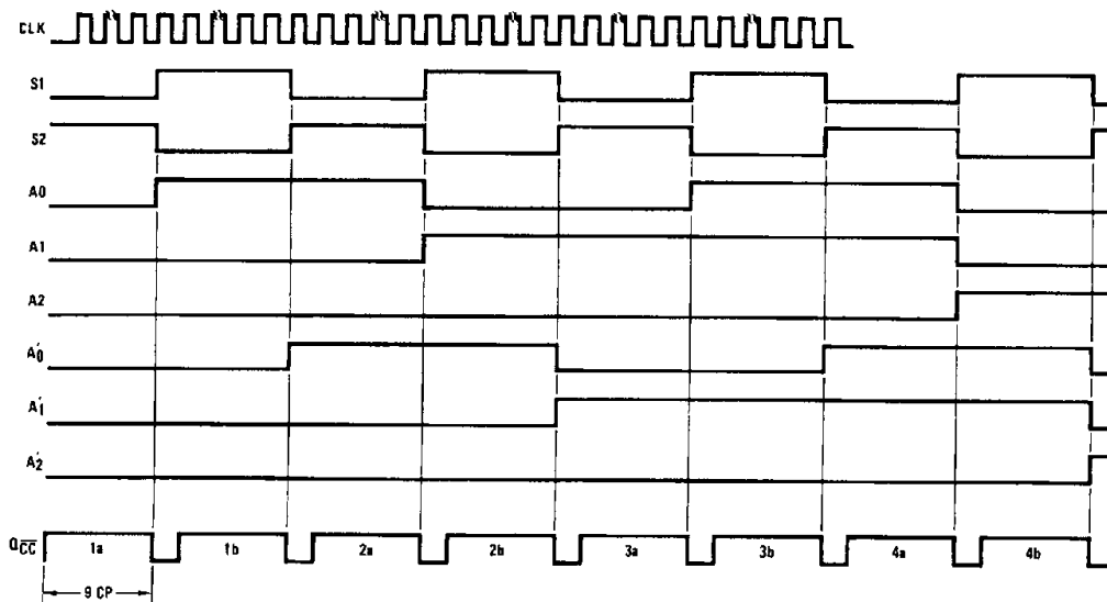
FIGURE 9b. Timing Diagram
