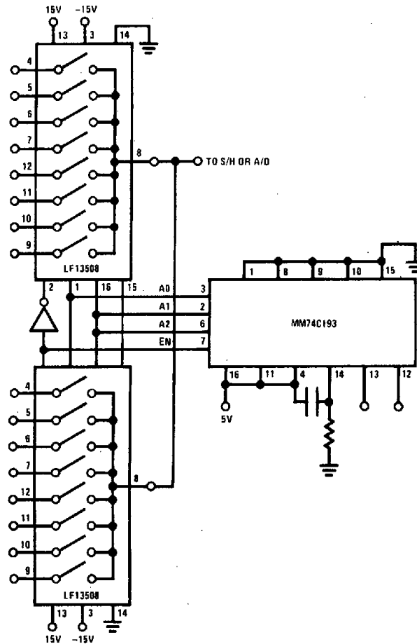
FIGURE 10. A 16-Channel Multiplexer with Sequential Multiplexing
