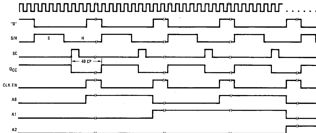
FIGURE 7a. Sequentially Multiplexed D/A with Sample and Hold
