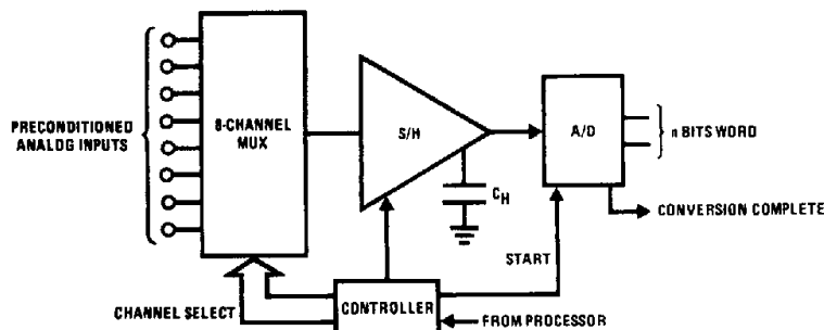
FIGURE 5. Random-Addressed, Multiplexed DAU
