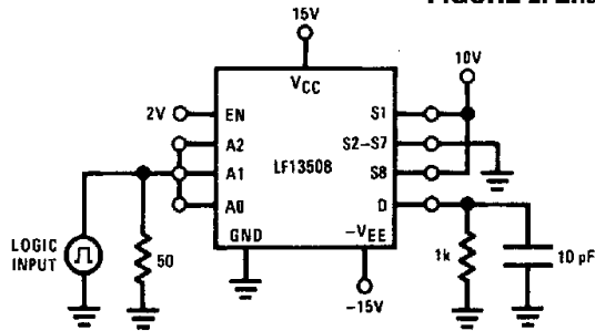
FIGURE 3. Break-Before-Make
