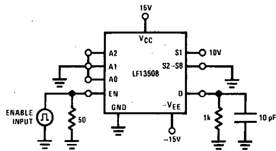
FIGURE 2. Enable Times
