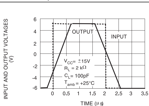
Figure 16. Voltage follower large signal pulse response
