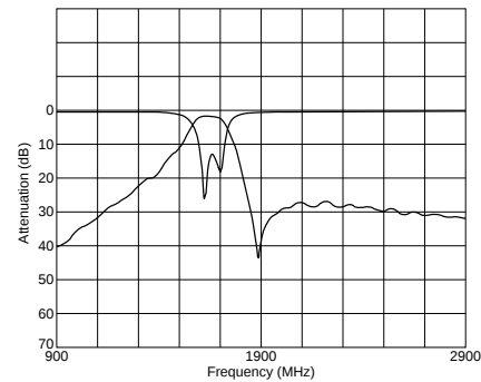
Frequency Characteristics
