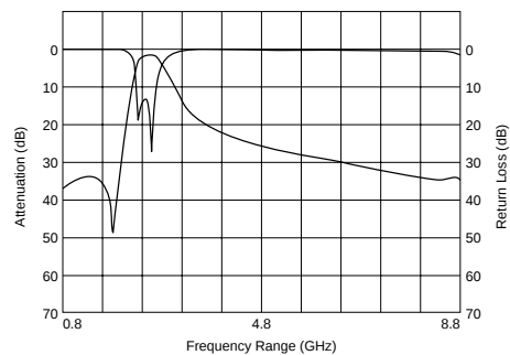
Frequency Characteristics
