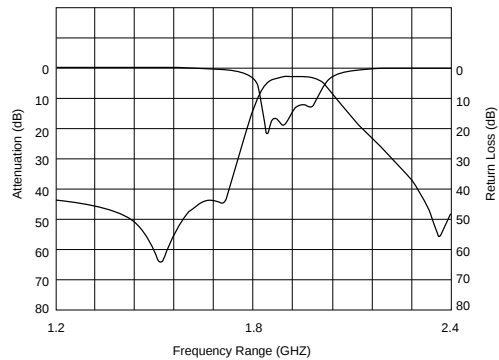
Frequency Characteristics
