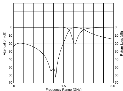
Frequency Characteristics
