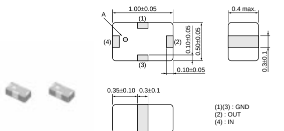
LFL15_TC Series
