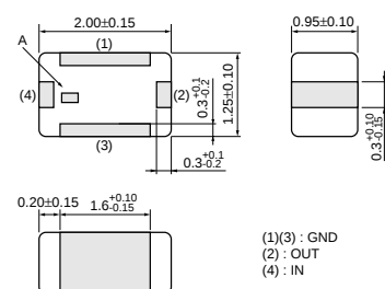
LFB21_SG Series
