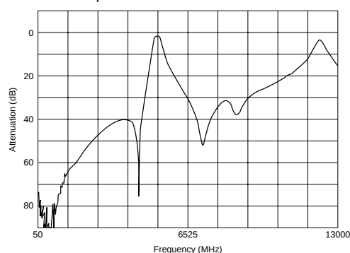
Spurious: DFCB25G25LAHAA
