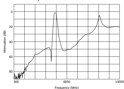
Spurious: DFCB35G25LAHAA
