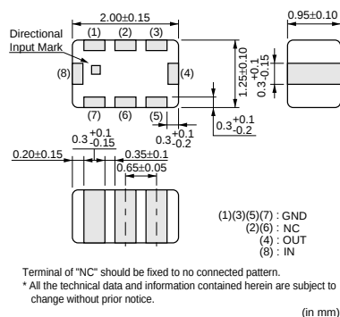
LFL21_TC Series
