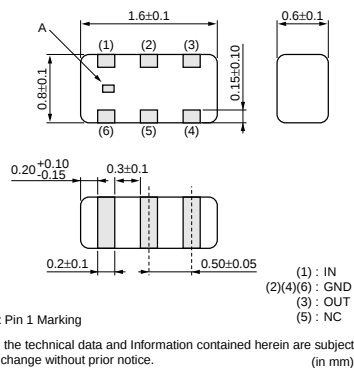
LFL18_TC Series
