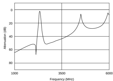
Spurious: DFCB32G33LBJAA
