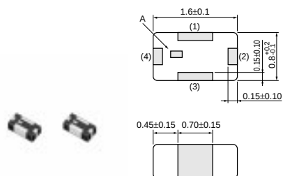
LFB18_SG Series
