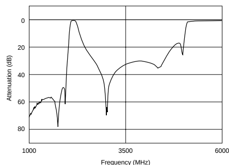
Spurious: DFCH32G14HDHA
