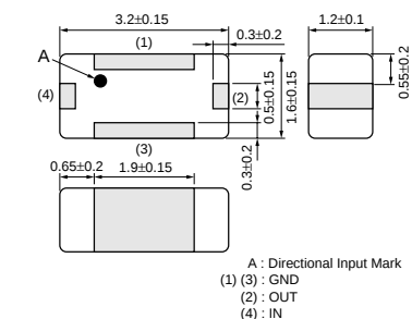
LFB31_SG Series
