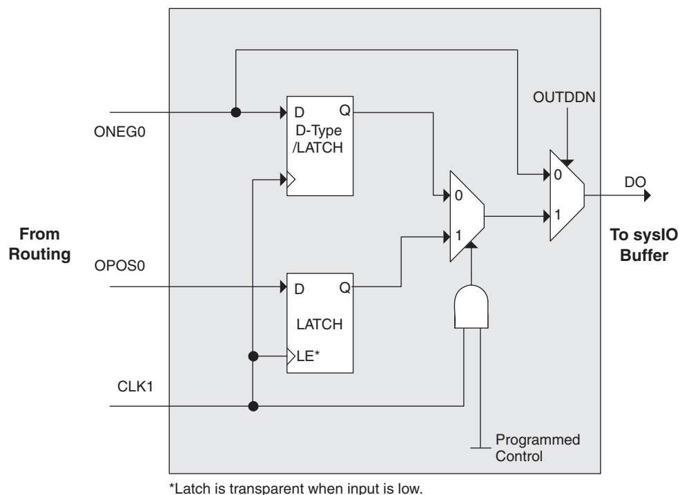
Figure 2-22. Output Register Block
