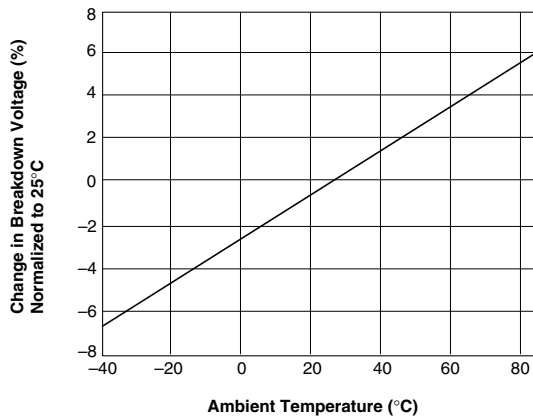
Figure 15. Switch Breakdown Voltage vs. Temperature
