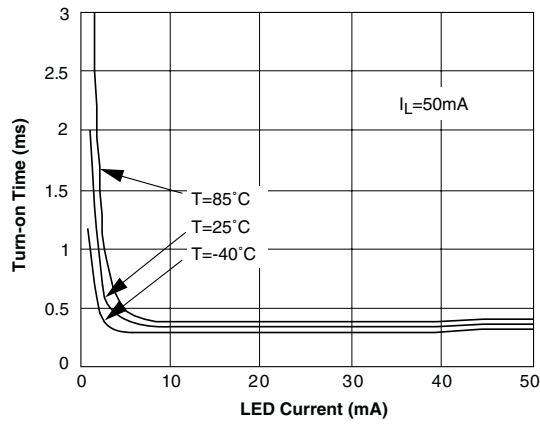
Figure 20. Turn-On Time vs. LED Current
