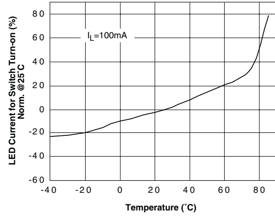
Figure 4. LED Current for Switch Turn-on vs. Temperature
