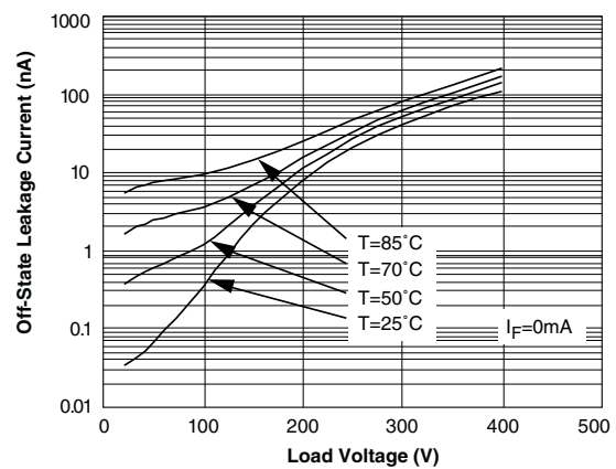
Figure 12. Leakage Current vs. Applied Voltage
