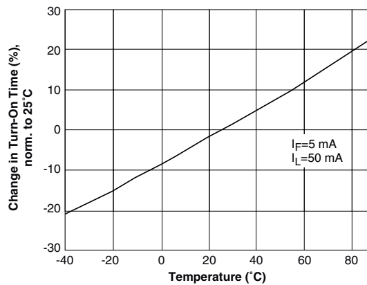
Figure 18. Turn-On Time vs. Temperature
