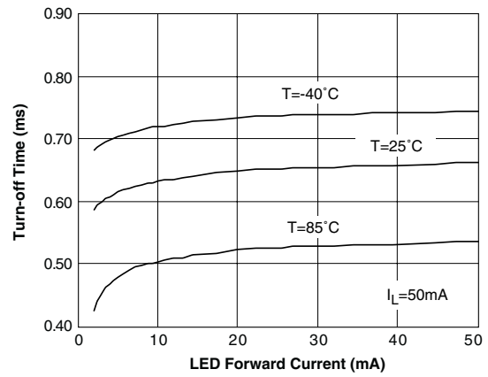
Figure 21. Turn-Off Time vs. LED Current
