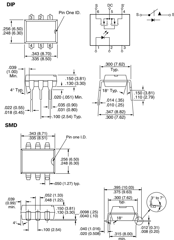
Package Dimensions in Inches (mm)
