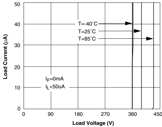
Figure 15. Switch Breakdown Voltage vs. Temperature
