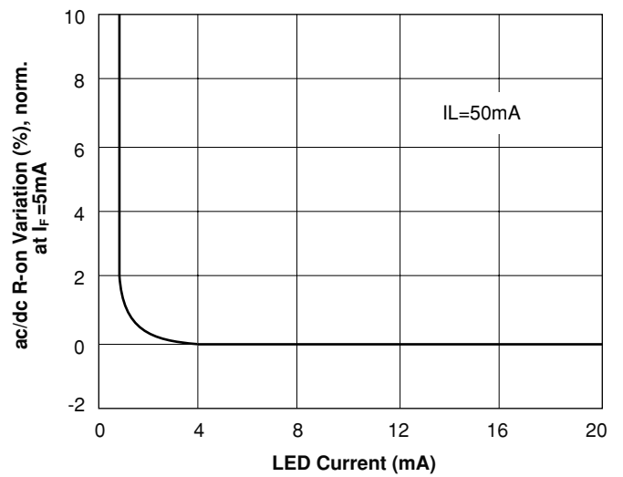
Figure 12. Variation in ON-resistance vs. LED Current
