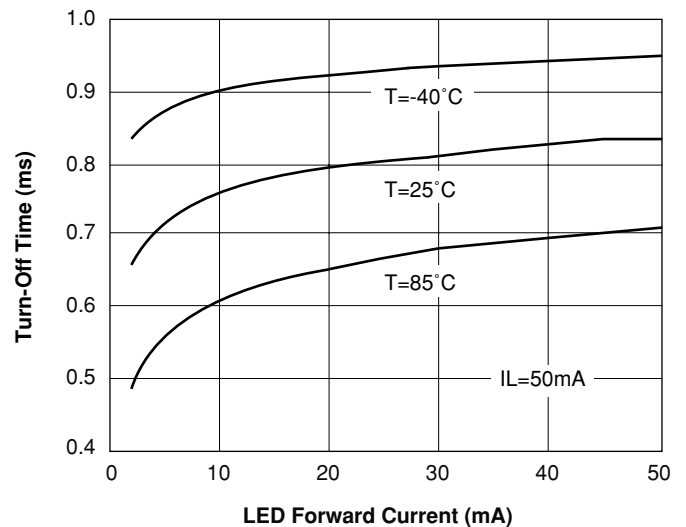
Figure 24. Turn-Off Time vs. LED Current
