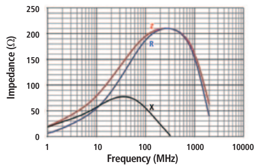
29F0330-2SR-10
