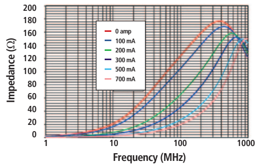
LI0603G121R-10
