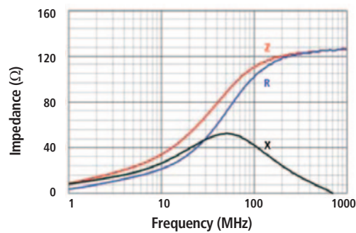
29F0318-1SR-10
