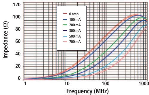
LI0603G800R-10
