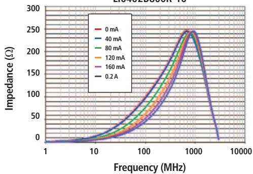
LI0402B800R-10
