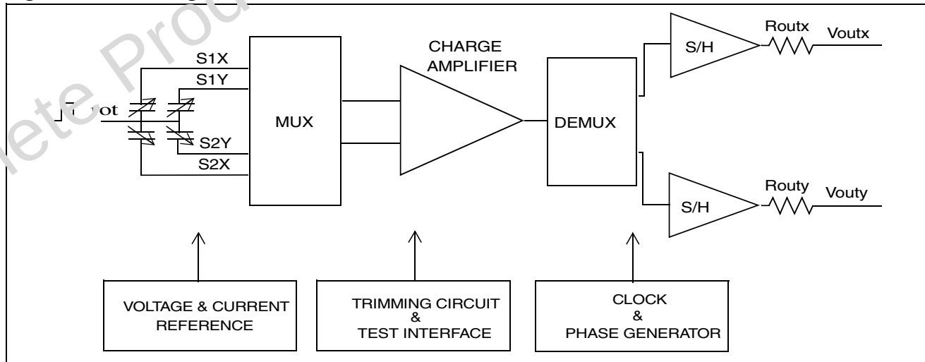
Figure 2. Block Diagram
