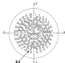
21-35 79 contacts size 22D
