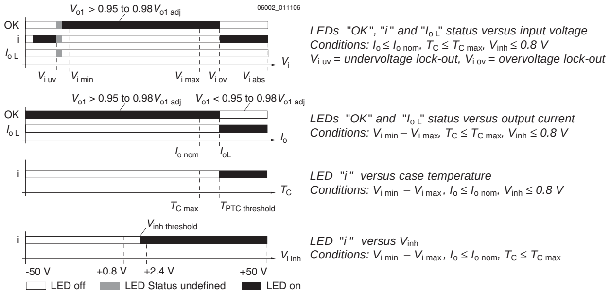
Fig. 23 LED indicators
