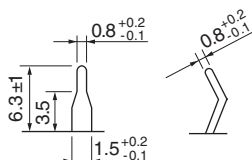
(Terminal dimensions)
