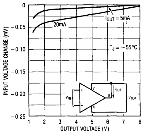
Shunt Gain
