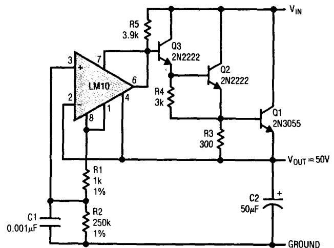
Floating Regulator
