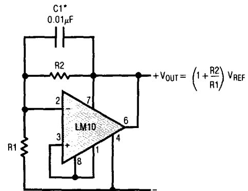
Shunt Regulator
