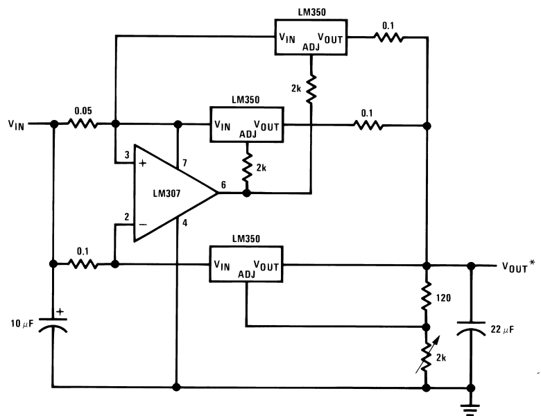
10A Regulator
