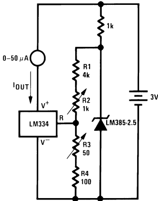
0°F–50°F Thermomemter
