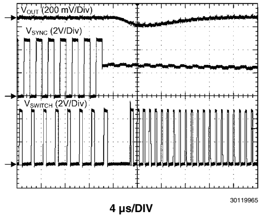
SYNC Signal Lost
