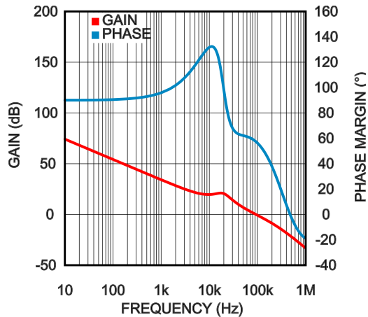
FIGURE 12. Loop Response
