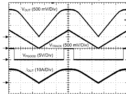
Startup with applied Track Signal
