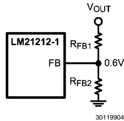
FIGURE 5. Setting V_{OUT}
