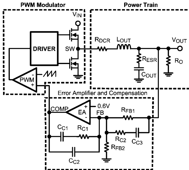
FIGURE 9. Loop Diagram
