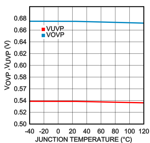
OVP/UVLP Threshold vs. Temperature
