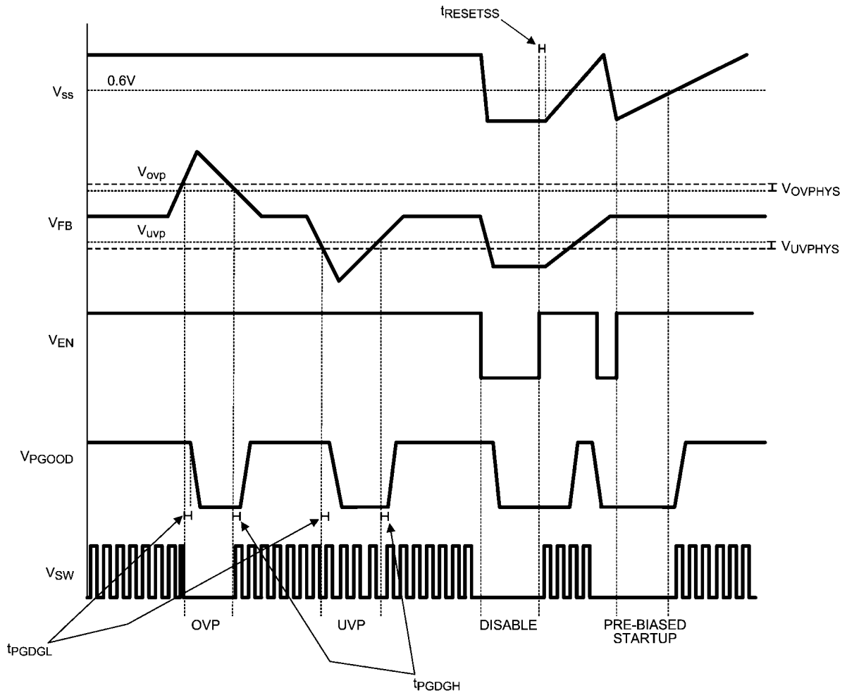
FIGURE 3. PGGOOD Conditions
