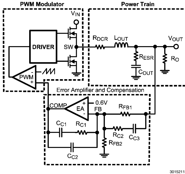
FIGURE 9. Loop Diagram
