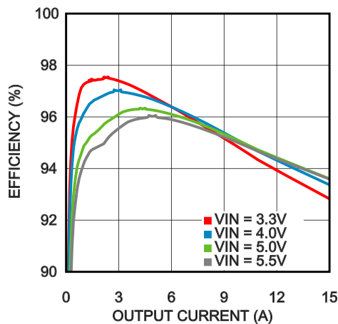
Efficiency ( V_{OUT} = 2.5V , f_{SW} = 500\text{ kHz} , Inductor P/N SER2010-601MLD)
