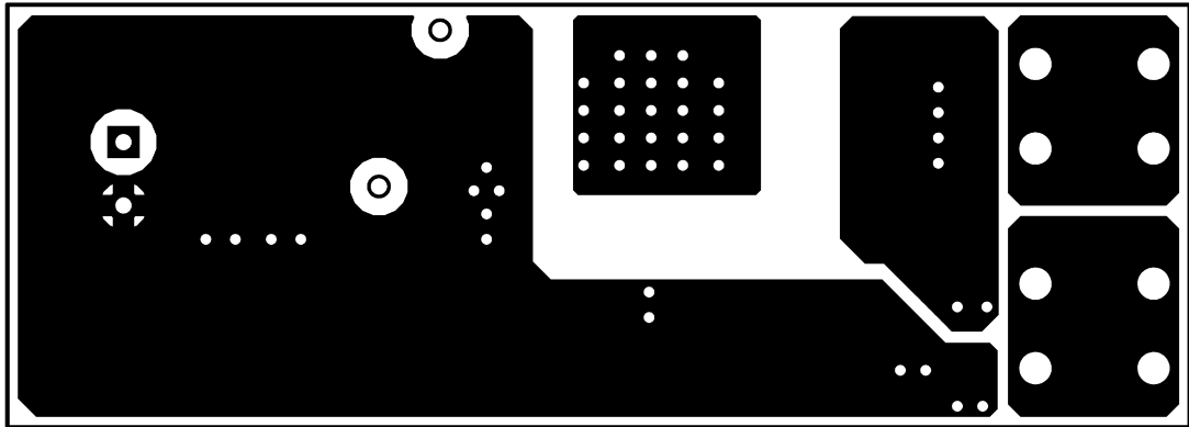
Figure 23. Solder Side
