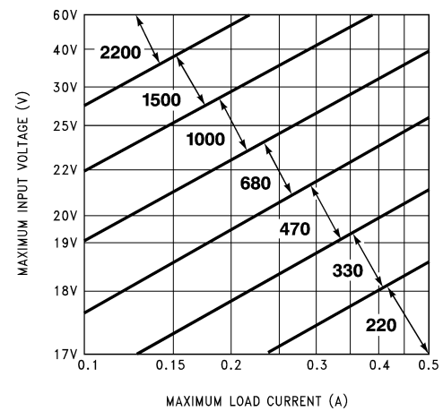
Figure 28. LM2574HV-15 Inductor Selection Guide
