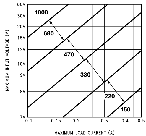
Figure 26. LM2574HV-5.0 Inductor Selection Guide
