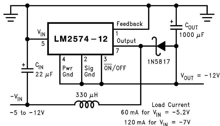
Figure 32. Negative Boost
