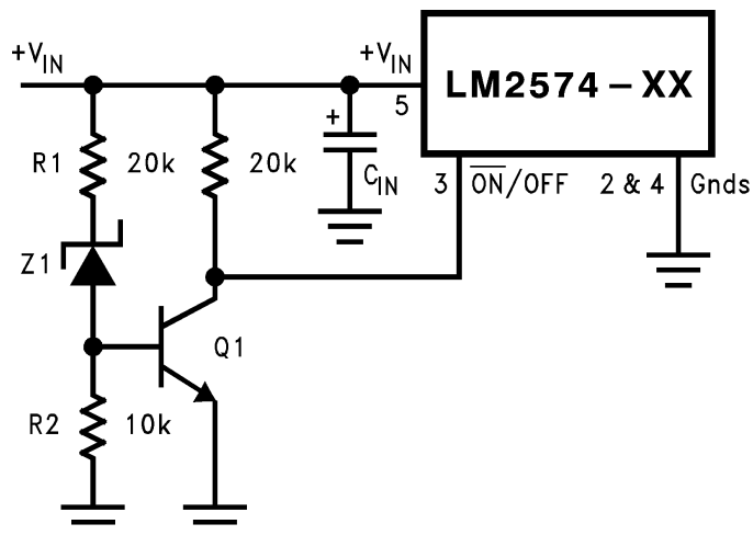
Figure 33. Undervoltage Lockout for Buck Circuit
