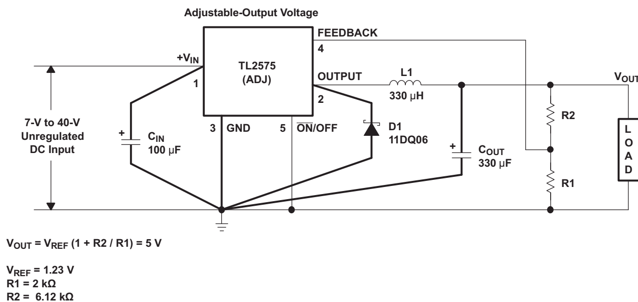
Figure 11. Test Circuits and Layout Guidelines
