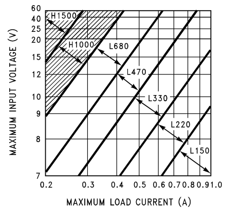
Figure 28. LM2575(HV)-5.0
