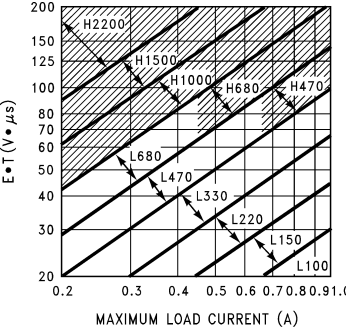
Figure 14. LM2575(HV)-ADJ
