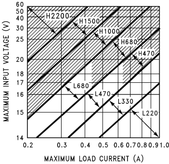
Figure 12. LM2575(HV)-12
