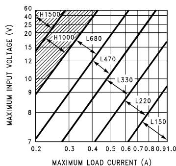
Figure 11. LM2575(HV)-5.0
