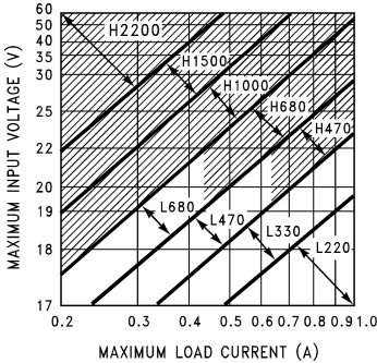
Figure 13. LM2575(HV)-15
