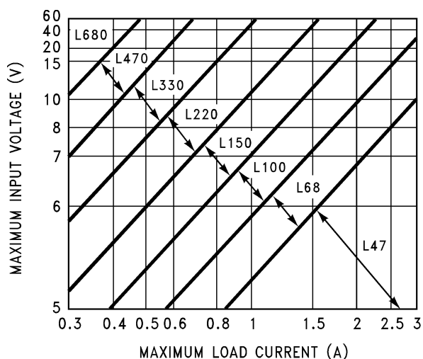
Figure 23. LM2576(HV)-3.3
