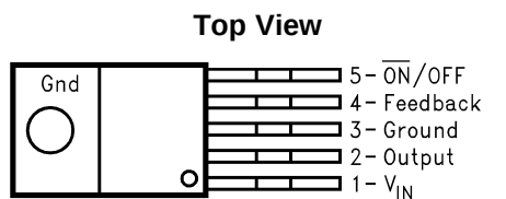
Figure 36. DPAK/TO-263 (S) Package 5-Lead Surface-Mount Package LM2576S-XX or LM2576HVS-XX See Package Number KTT0005B LM2576SX-XX or LM2576HVSX-XX See Package Number KTT0005B
