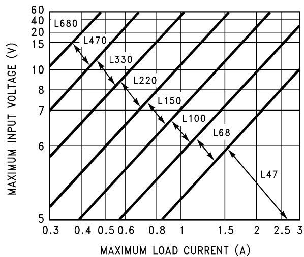
Figure 23. LM2576(HV)-3.3
