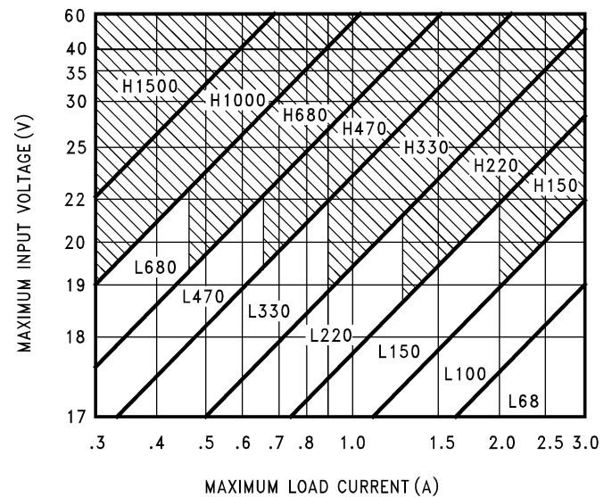
Figure 26. LM2576(HV)-15
