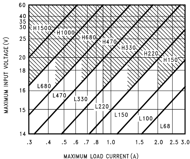
Figure 25. LM2576(HV)-12
