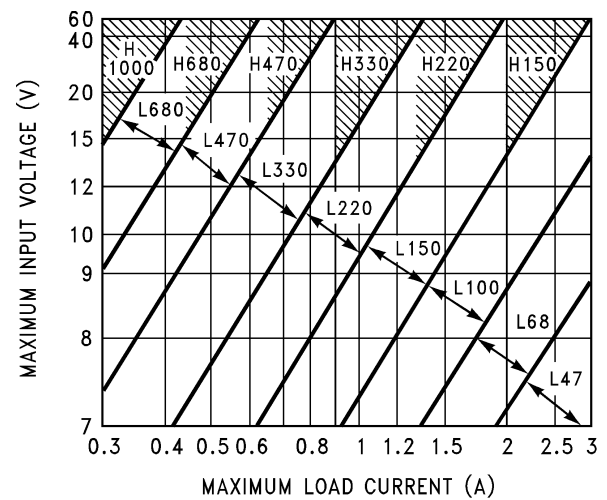
Figure 24. LM2576(HV)-5.0
