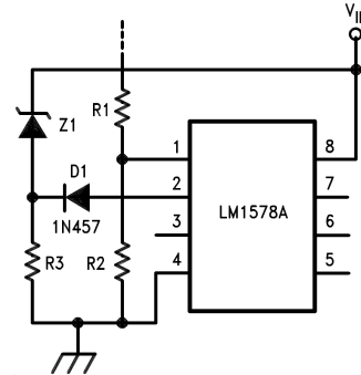
FIGURE 8. Under-Voltage Lockout
