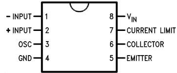
Dual-In-Line Package
