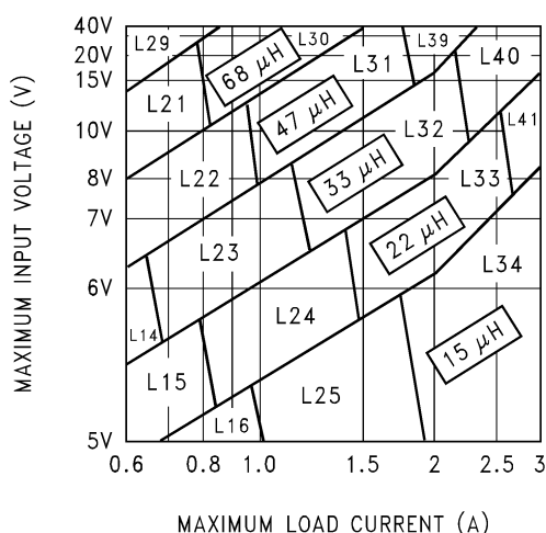
Figure 21. LM2596-3.3
