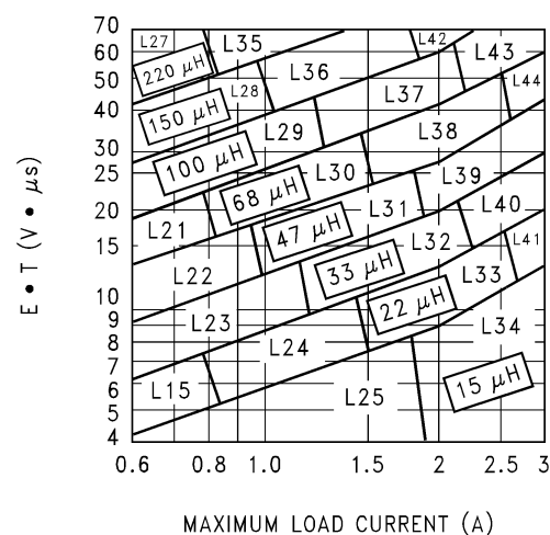
Figure 24. LM2596-ADJ
