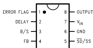
Figure 1. 8-Lead DIP (N) Top View
