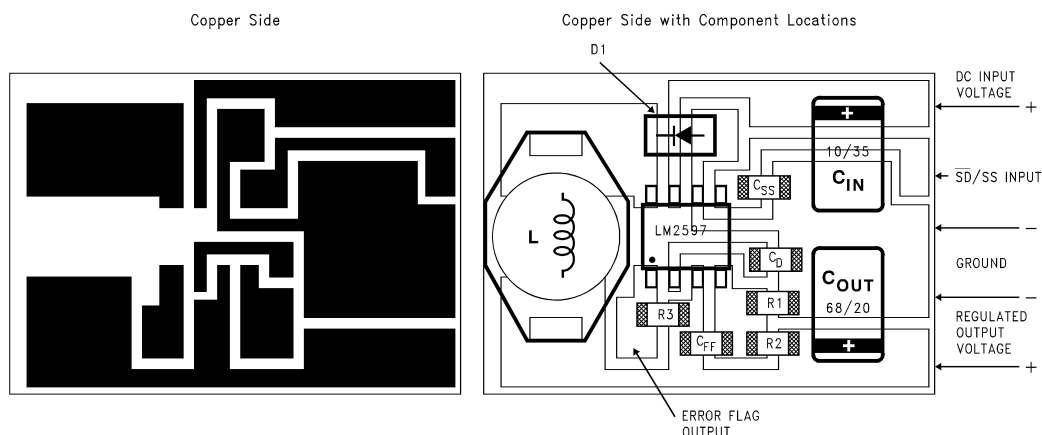
Figure 36. TYPICAL SURFACE MOUNT PC BOARD LAYOUT, ADJUSTABLE OUTPUT (2X size)
