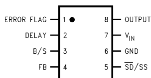
Figure 2. 8-Lead Surface Mount (M) Top View
