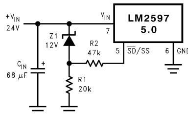
Figure 31. Undervoltage Lockout for a Buck Regulator
