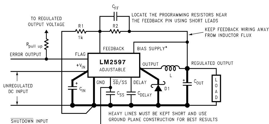
Figure 11. Fixed Output Voltage Versions
