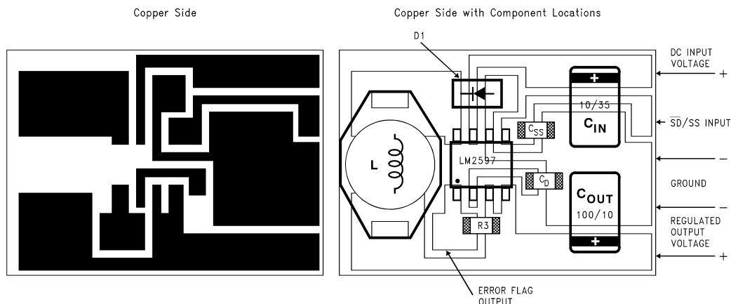
Figure 35. TYPICAL SURFACE MOUNT PC BOARD LAYOUT, FIXED OUTPUT (2X size)
