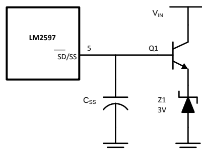
Figure 15. External 3.7V Soft-Start Clamp
