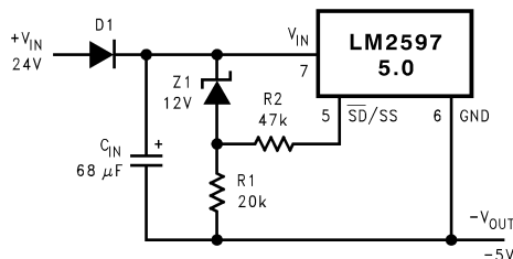
Figure 33. Undervoltage Lockout With Hysteresis for an Inverting Regulator
