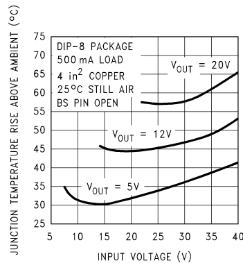
Figure 22. Junction Temperature Rise, DIP-8
