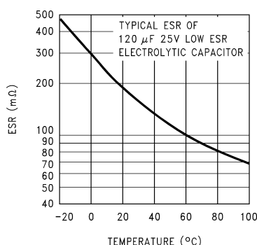
Figure 18. Capacitor ESR Change vs Temperature
