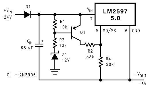
Figure 32. Undervoltage Lockout Without Hysteresis for an Inverting Regulator
