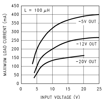
Figure 30. Maximum Load Current for Inverting Regulator Circuit
