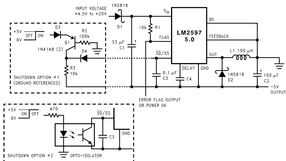
Figure 29. Inverting -5V Regulator With Shutdown and Soft-start
