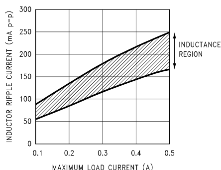
Figure 21. Peak-to-Peak Inductor Ripple Current vs Load Current
