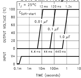
Soft-start Response
