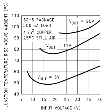
Figure 23. Junction Temperature Rise, SO-8
