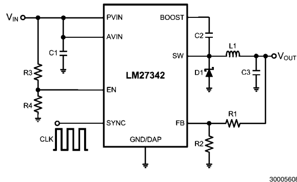
FIGURE 5. Resistor Divider on EN
