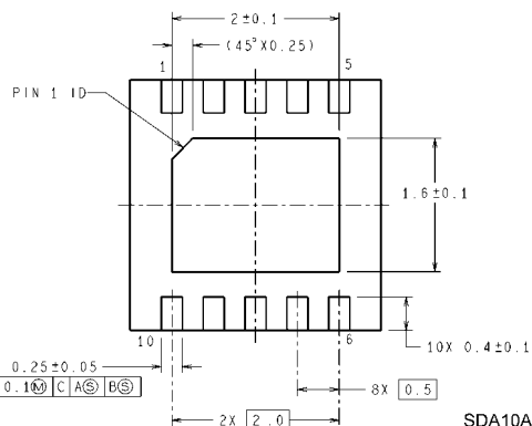
10-Lead LLP Package NS Package Number SDA10A
