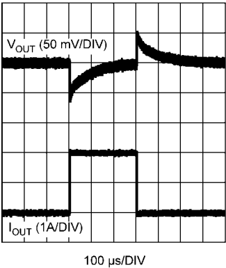
Transient Response I_{OUT} = 100\text{ mA} - 2\text{ A} @ slewrte = 2\text{ A} / \mu\text{s}
