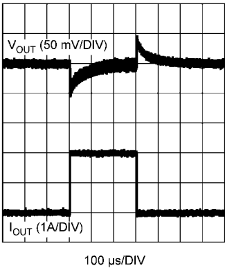
Transient Response I_{OUT} = 100\text{ mA} - 2\text{ A} @ \text{slewrates} = 2\text{ A} / \mu\text{s}
