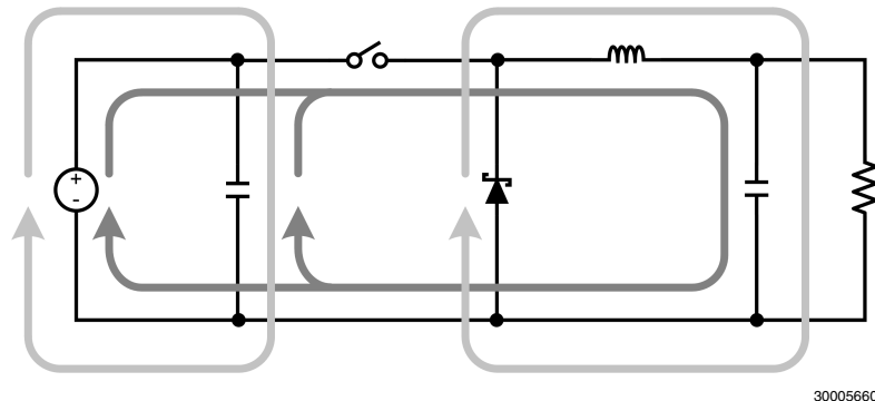
FIGURE 9. Buck Converter Current Loops
