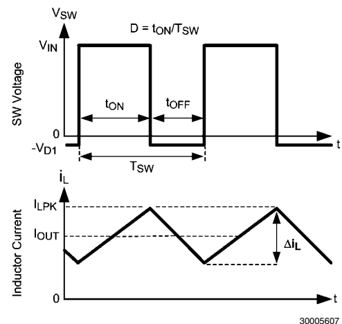
FIGURE 2. LM27341/LM27342 Waveforms of SW Pin Voltage and Inductor Current
