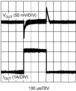
Transient Response I_{OUT} = 100\text{ mA} - 2\text{ A} @ \text{slewrte} = 2\text{ A} / \mu\text{s}
