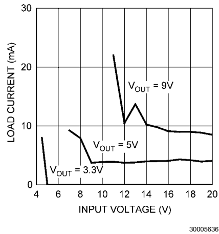
FIGURE 4. Minimum Load Current for L = 1.5 \mu\text{H}
