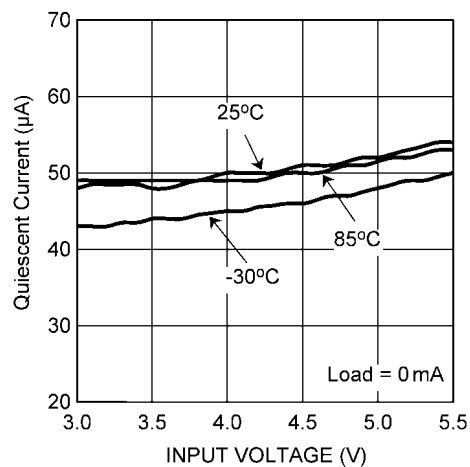
Operating Supply Current
