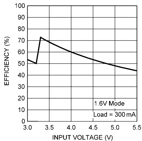
Efficiency vs. Input Voltage, 1.6V Mode
