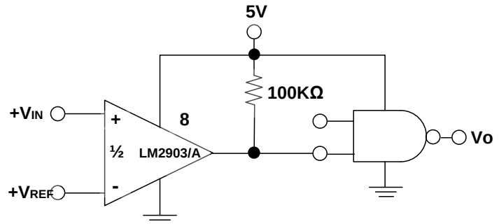
Driving CMOS
