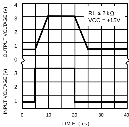
Figure 5: Voltage follower pulse response
