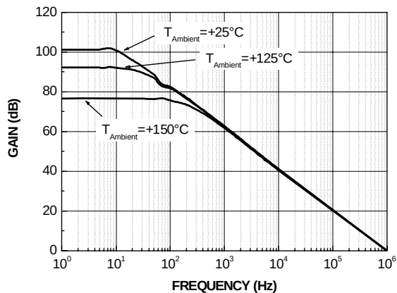
Figure 3: Open loop frequency response
