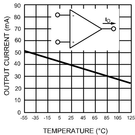
Figure 10: Current limiting
