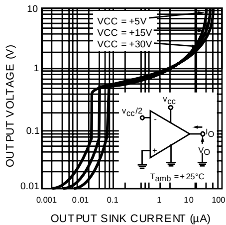
Figure 9: Output characteristics (sink)
