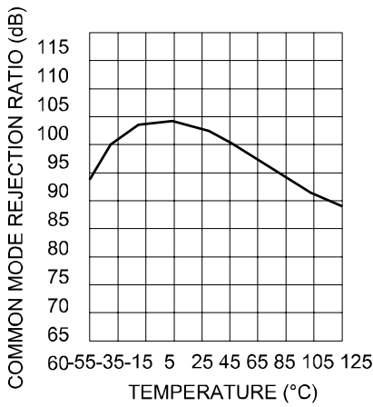
Figure 16: Common mode rejection ratio versus temperature
