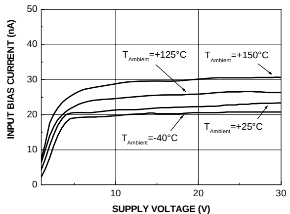
Figure 6: Input bias current
