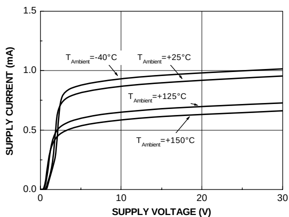
Figure 7: Supply current
