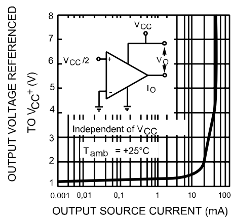
Figure 8: Output characteristics
