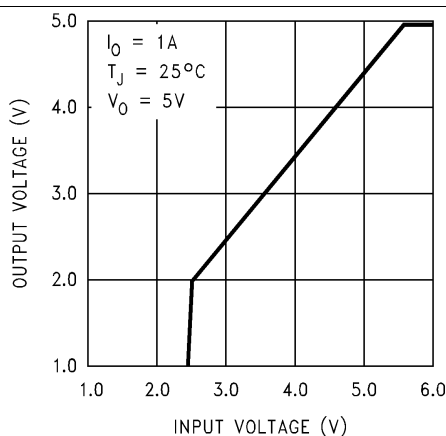
Figure 28. Low Voltage Behavior
