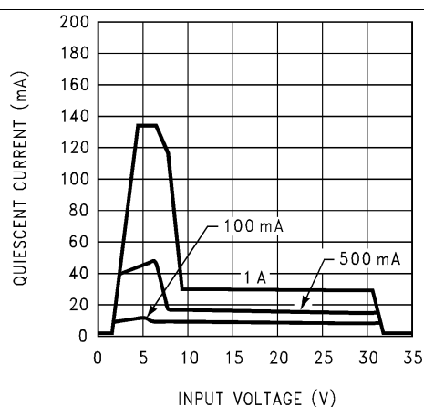
Figure 5. Quiescent Current
