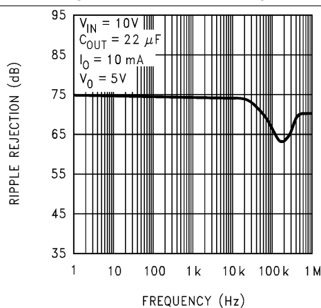
Figure 9. Ripple Rejection
