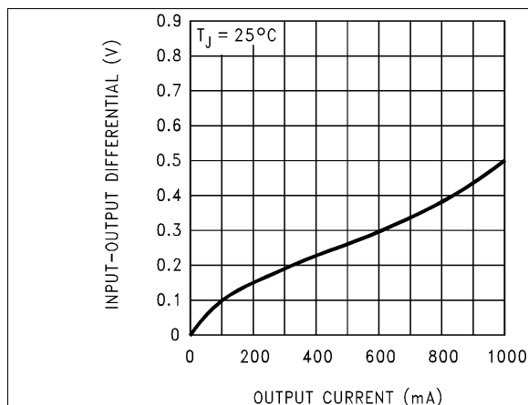
Figure 1. Dropout Voltage
