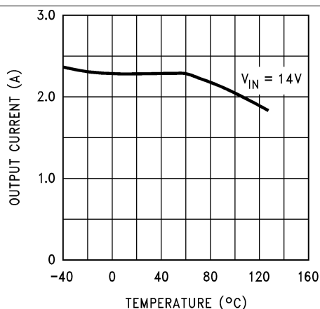
Figure 21. Peak Output Current
