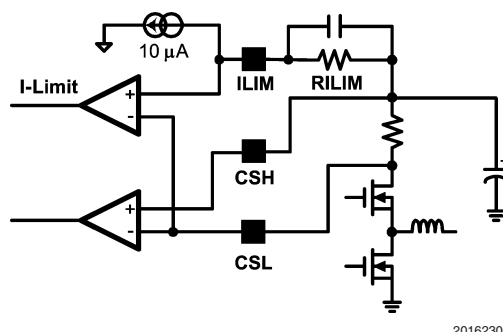
FIGURE 2. Current Sensing by External Sense Resistor
