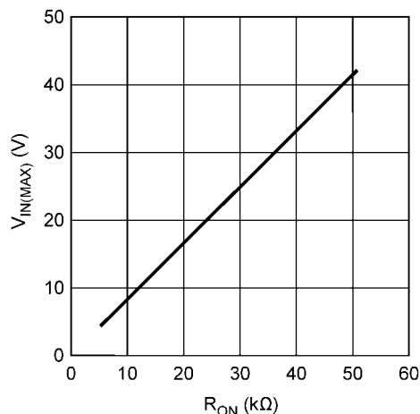
FIGURE 4. Maximum V_{IN} for selected R_{ON}
