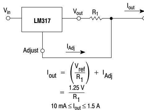
Figure 26. Current Regulator
