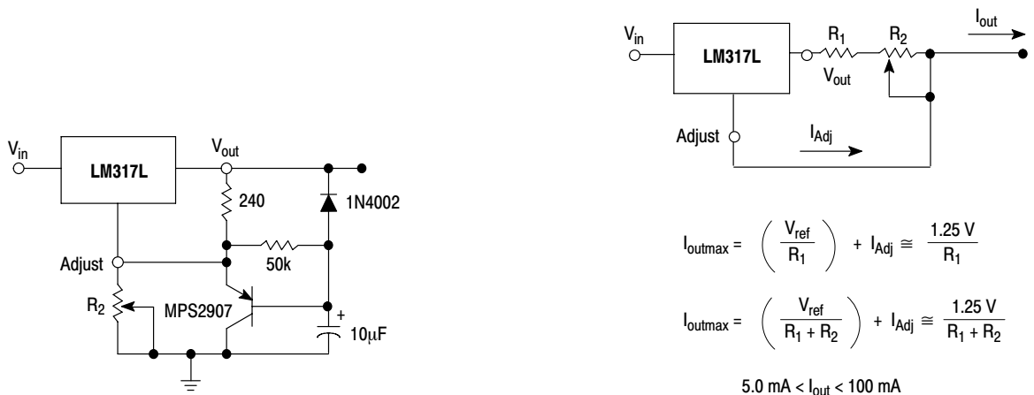
Figure 21. Slow Turn-On Regulator
