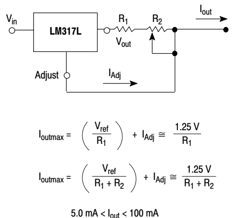
Figure 22. Current Regulator
