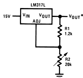
Figure 32. 1.2V–12V Regulator with Minimum Program Current
