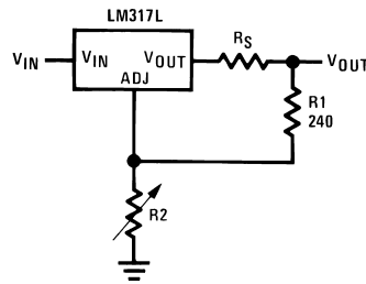
Figure 17. Regulator with Line Resistance in Output Lead
