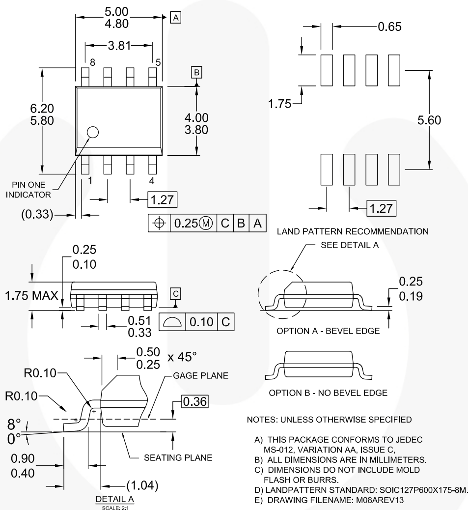
Figure 7. 8-Lead, SOIC, JEDEC MS 0-12, 0.150 inch Narrow Body
