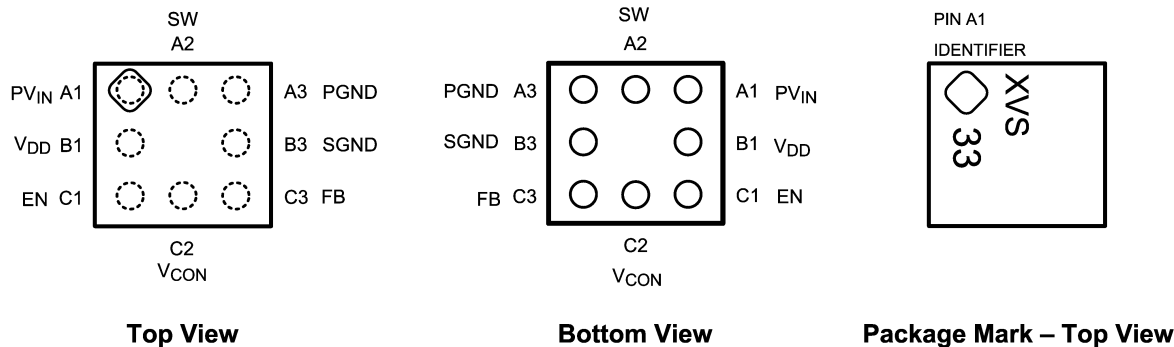
8-Bump Thin Micro SMD Package, Large Bump NS Package Number TLA08GNA
