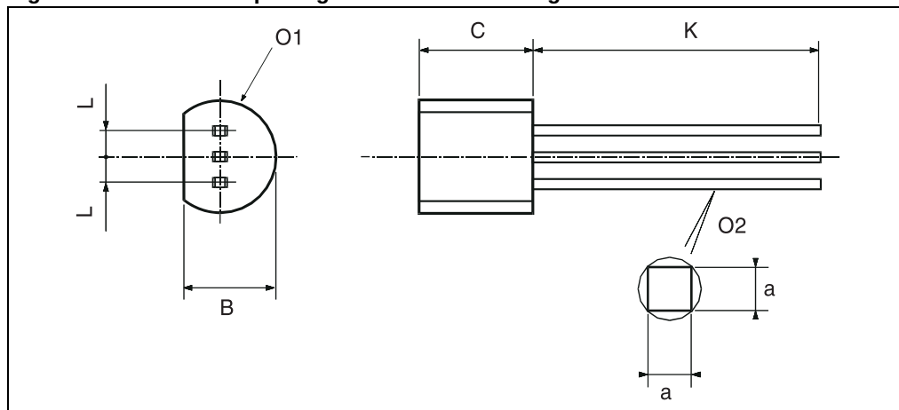
Figure 24. TO-92 bulk package mechanical drawing
