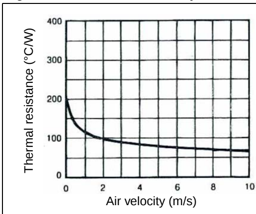
Figure 8. Thermal resistance junction to air
