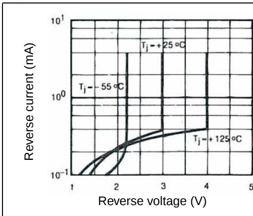
Figure 4. Reverse characteristics
