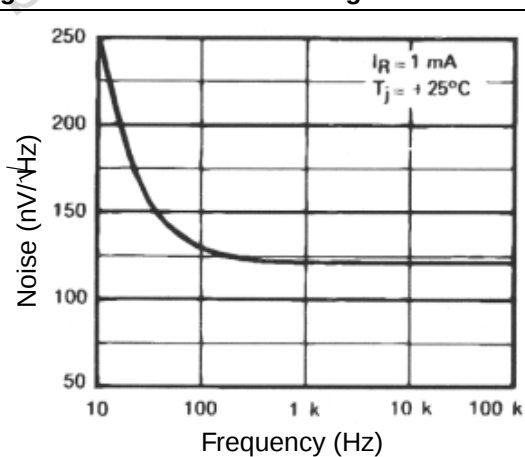
Figure 3. Zener noise voltage
