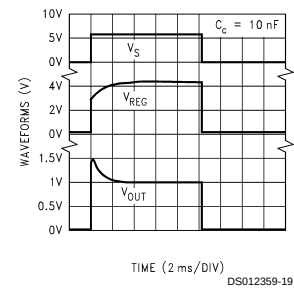
Response Time for 4.2V Version
