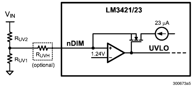
FIGURE 14. UVLO Circuit
