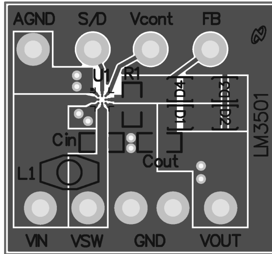
FIGURE 3. Evaluation Board Layout (2X Magnification) Top Layer
