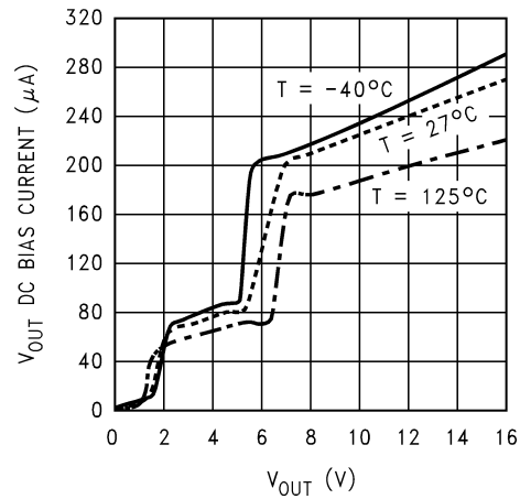
V_{OUT} DC Bias vs. V_{OUT} Voltage (LM3501-16)
