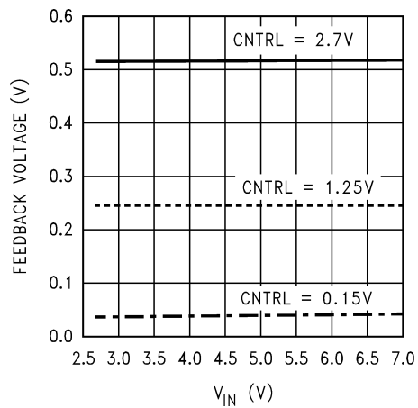
FB Voltage vs. V_{IN}
