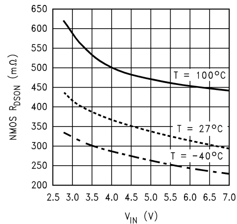
NMOS R_{DS(on)} vs. V_{IN} ( I_{SW} = 300\text{ mA} )
