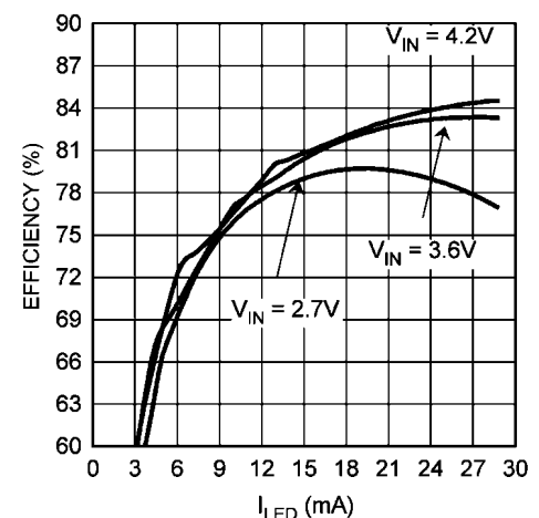
3 LED Efficiency vs I_{LED} ( L = \text{TDK VLF3012AT-220MR33} , R_L = 0.66\Omega )
