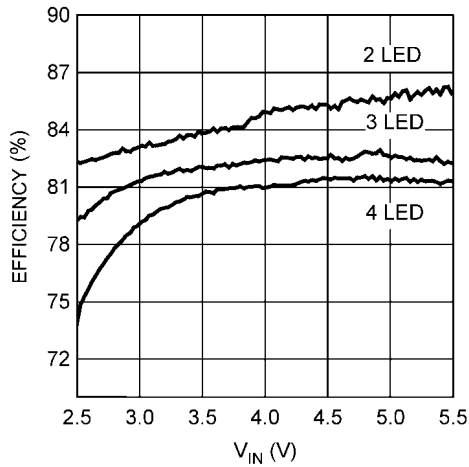
Efficiency vs V_{IN} ( I_{LED} = 20\text{mA} )
