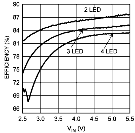
Efficiency vs V_{IN} ( I_{LED} = 30\text{mA} )
