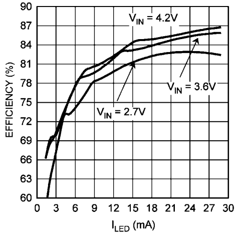
2 LED Efficiency vs I_{LED} ( L = \text{TDK VLF3012AT-220MR33} , R_L = 0.66\Omega )
