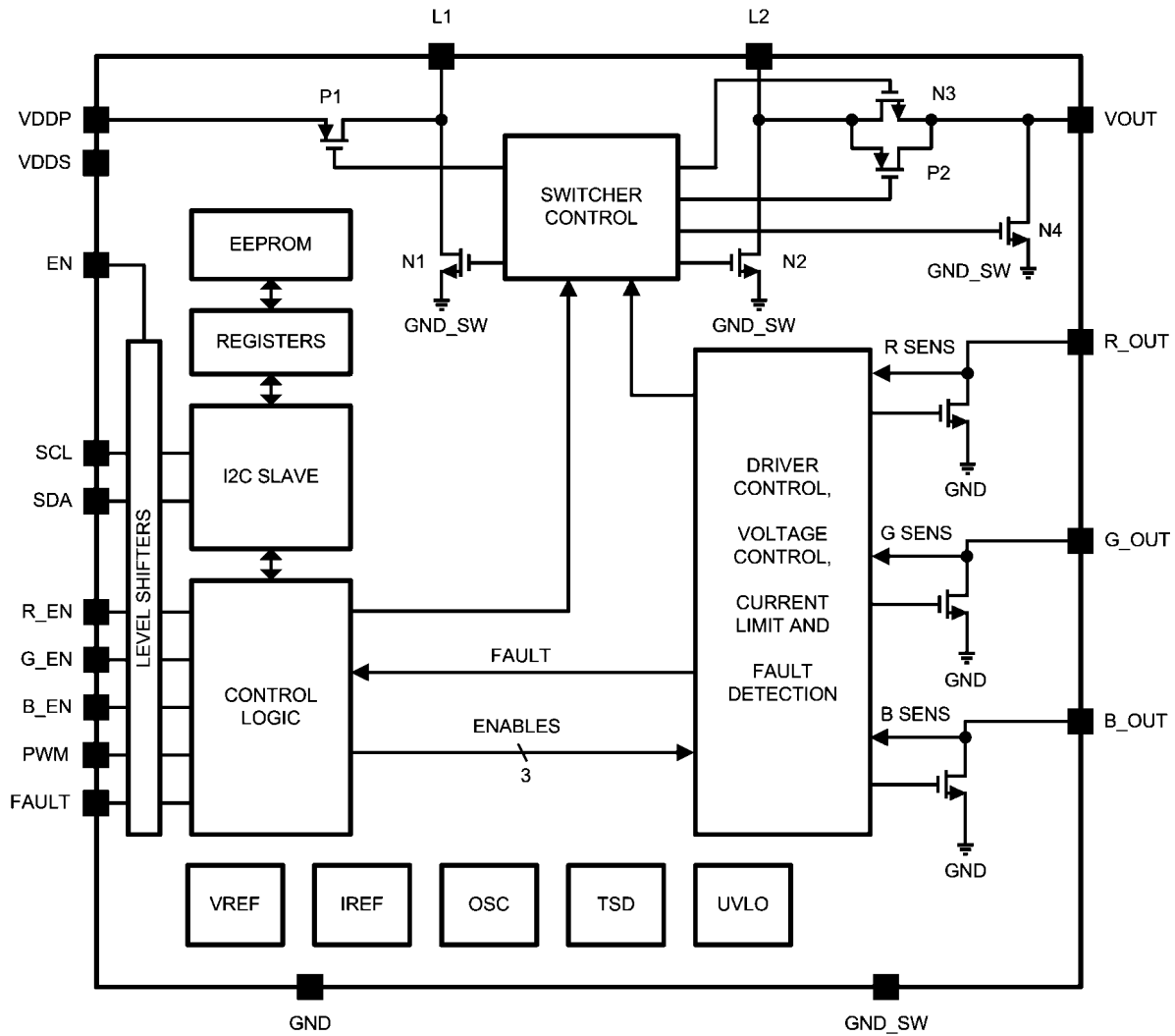
FIGURE 2. LM3549 Block Diagram
