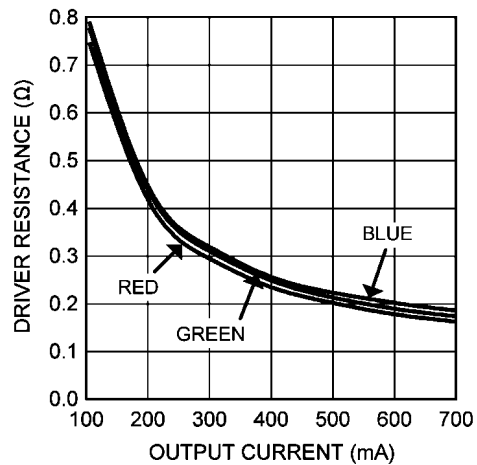
LED Driver Resistance vs Output Current ( V_{IN} = 3.8V )
