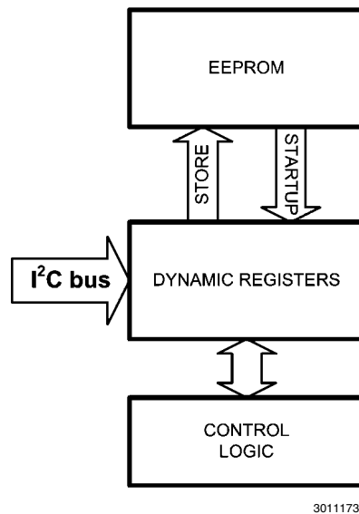
FIGURE 6. Register Structure
