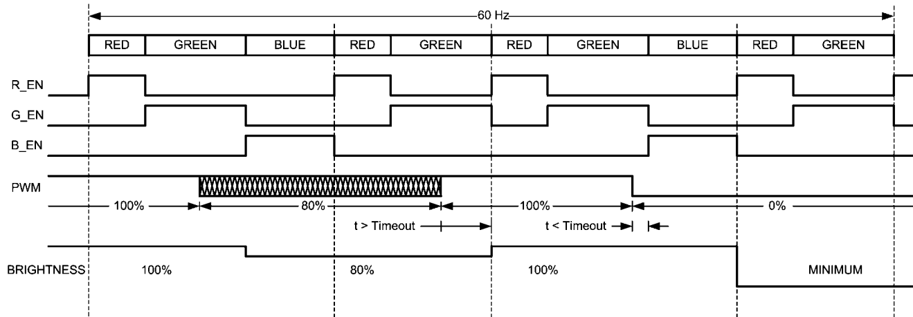
FIGURE 7. PWM Timing
