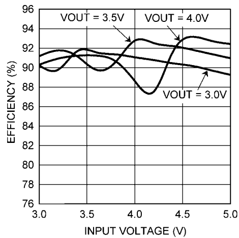
LED Drive Efficiency vs Input Voltage ( I_{OUT} = 300\text{ mA} )
