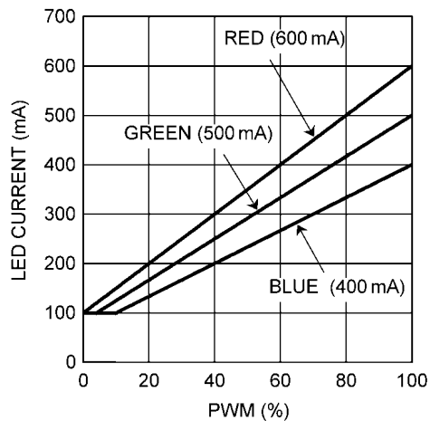
PWM Output Current Control
