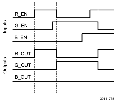
FIGURE 5. Control Signals
