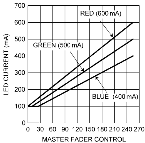
Master Fader Register Current Control
