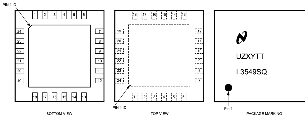
FIGURE 1. 24-Pin LLP Package, No Pullback
