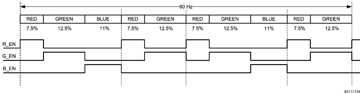
FIGURE 4. Timing Chart
