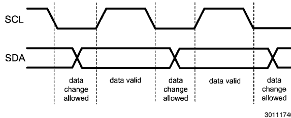
FIGURE 10. I 2 C Signals: Data Validity
